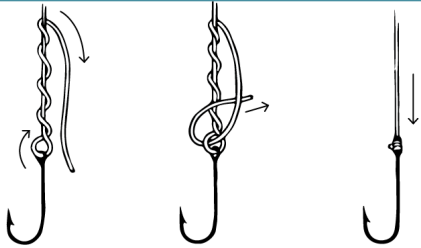
CLINCH KNOT
